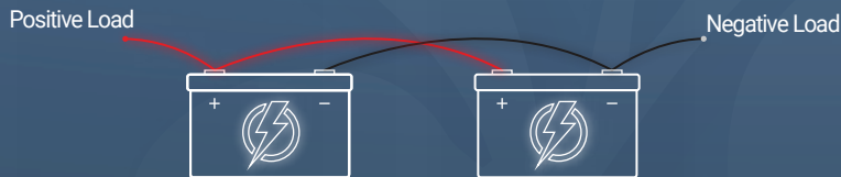
Parallel Connection 12V 150Ah Bank Increases Ah, Voltage stays the same.
